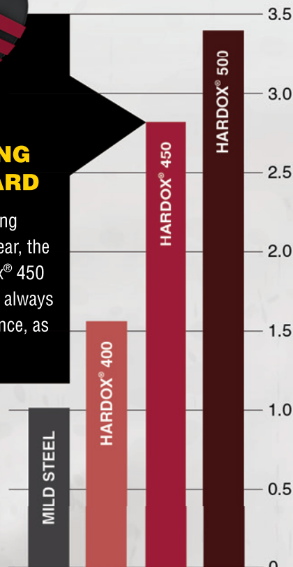
Relative useful life. Comparison between mild steel, Hardox® 400, Hardox® 450 and Hardox® 500.
