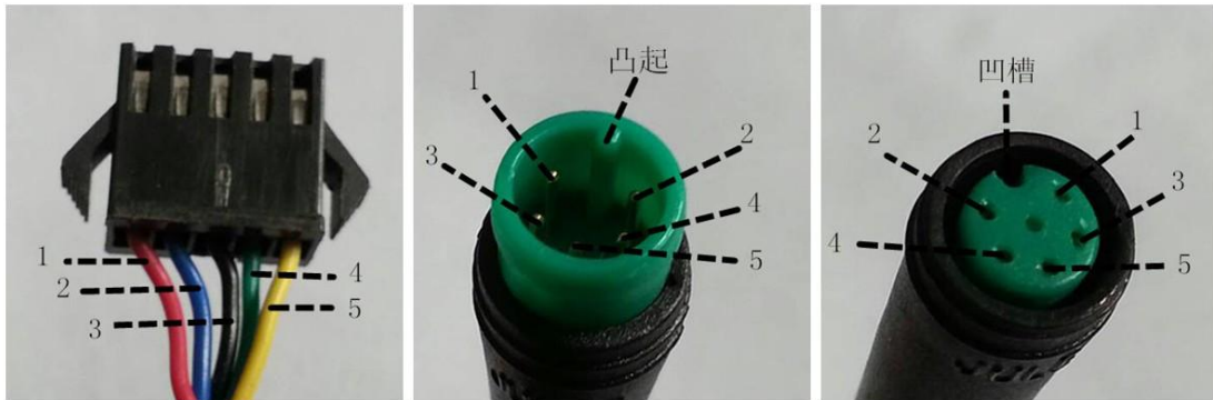
Controller connector
