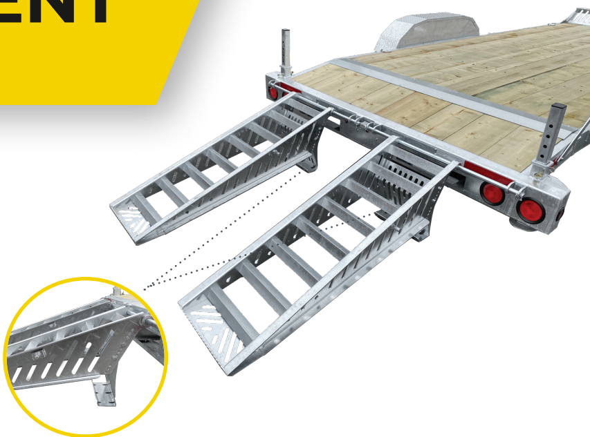
REINFORCED RAMPS WITH ADJUSTABLE HEEL
